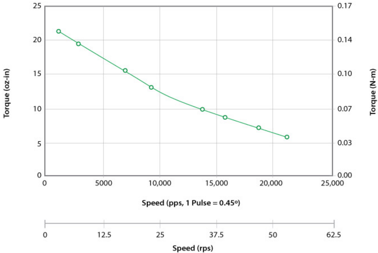
ZN417-17-02 (0.9° Step Motor) 24VDC, 1.96 Amp Peak, Bipolar, 1/2 Stepping
