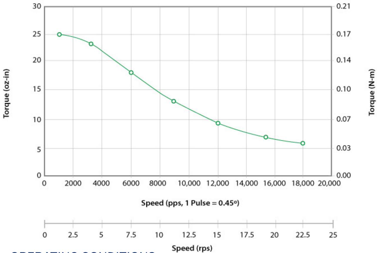
ZH417-17-03 (0.9° Step Motor) 24VDC, 1.54 Amp Peak, Bipolar, 1/2 Stepping
