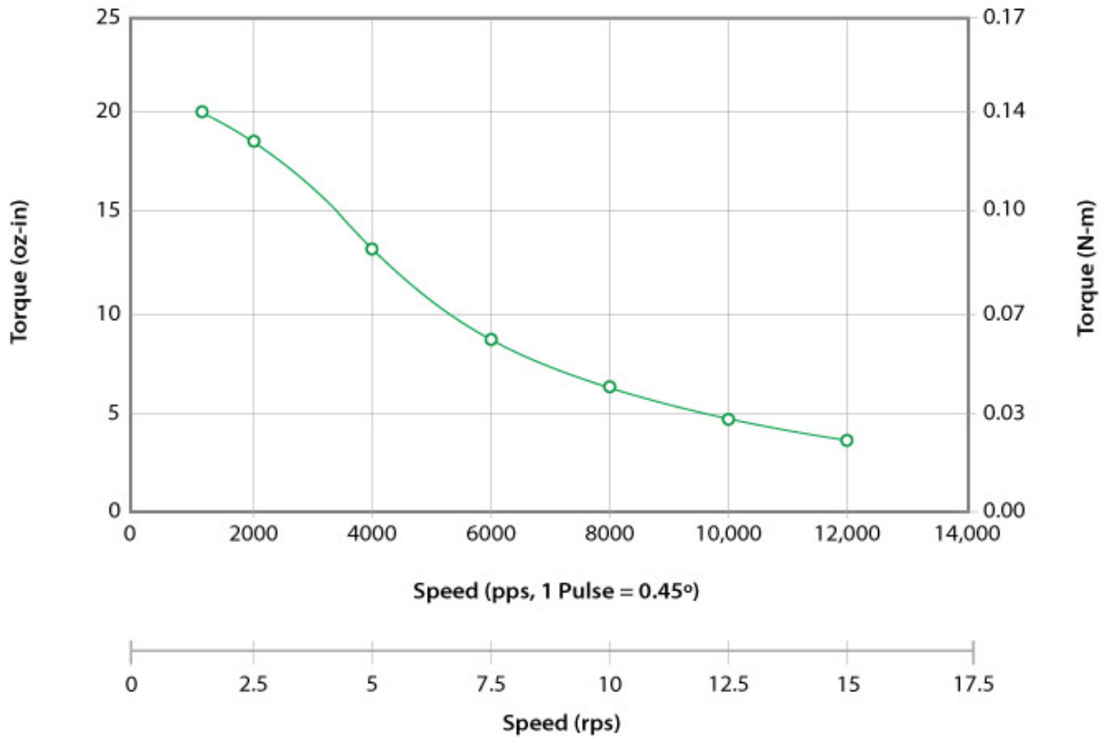
ZH417-17-01 (0.9° Step Motor) 24VDC, 0.7 Amp Peak, Bipolar, 1/2 Stepping
