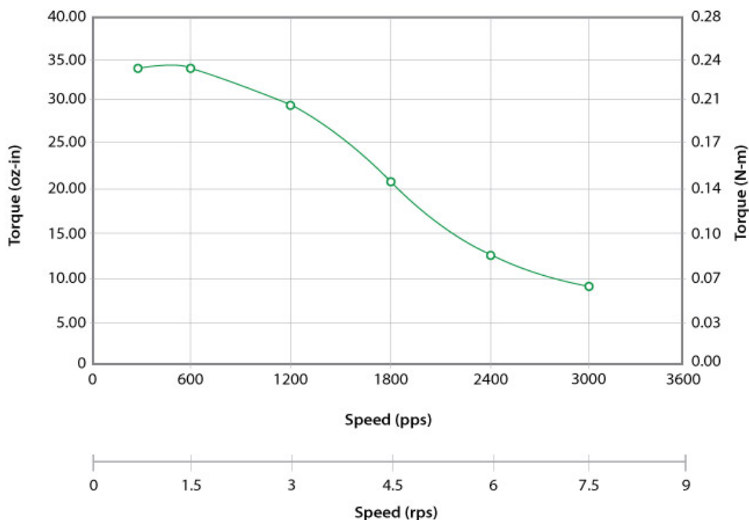
G4518S-02 24VDC, 0.4 Amps/Phase, Bipolar, 1/2 Stepping
