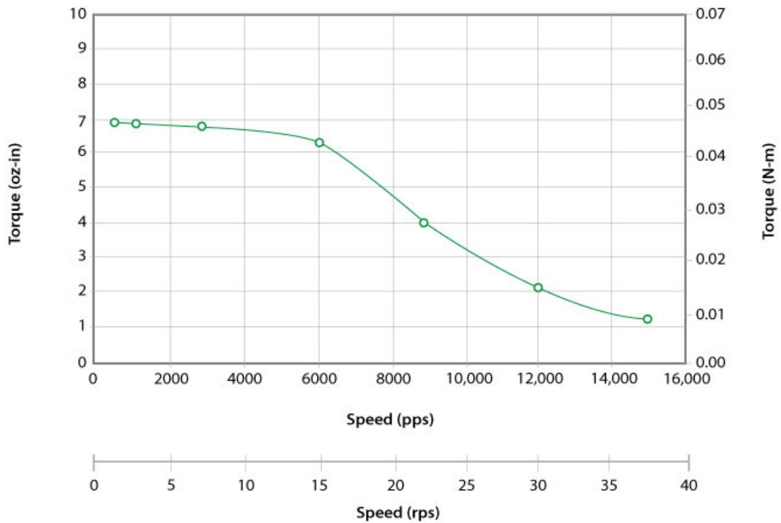
3518X-08 24VDC, 0.35 Amps/Phase, Bipolar, 1/2 Stepping
