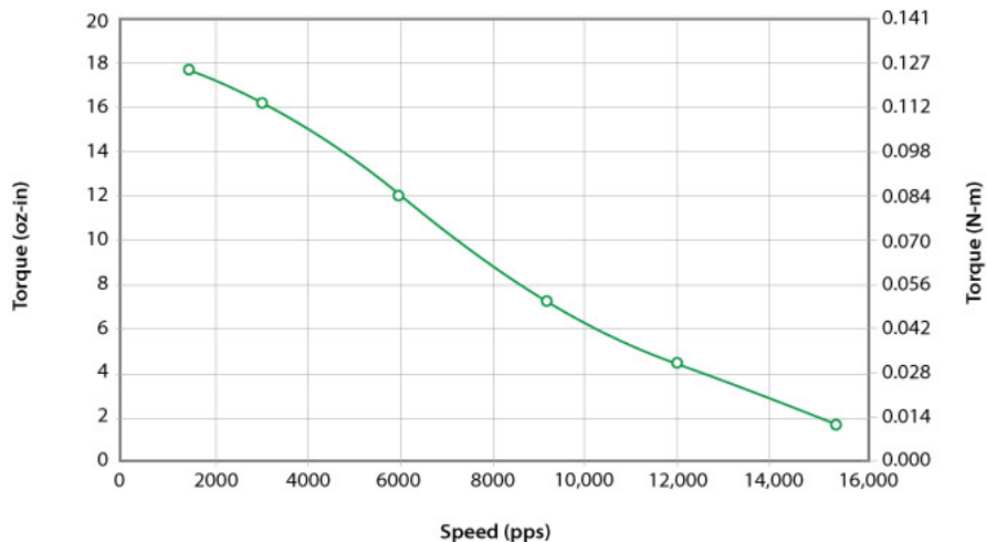
211-20-01 24VDC, 0.67 Amps/Phase, Bipolar, 1/2 Stepping
