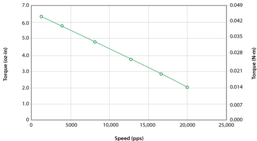
211-13-01 24VDC, 0.67 Amps/Phase, Bipolar, 1/2 Stepping
